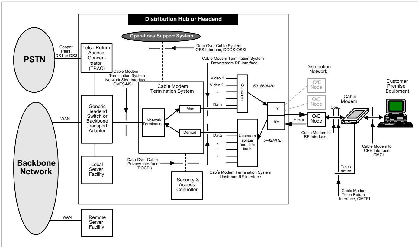
Figure 1-2. Data-over-Cable Reference Architecture
