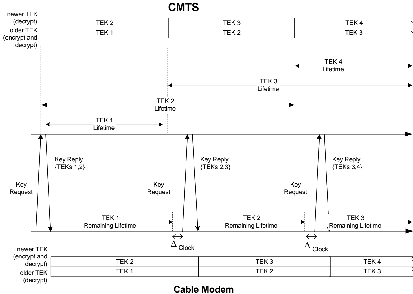
Figure 6-2. TEK Management in CMTS and CM
